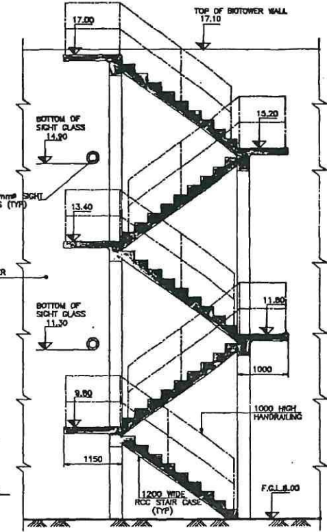
DETAILS OF RCC STAIR CASE (SCALE 1:50)
