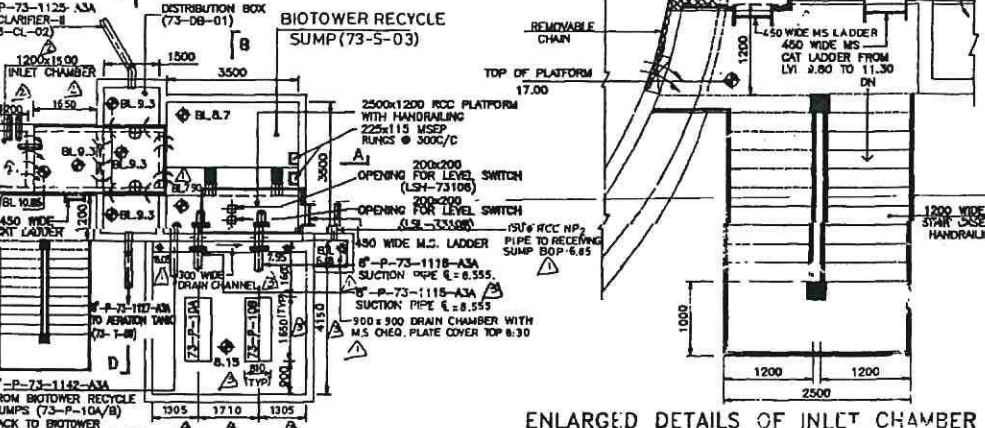
ENLARGED DETAILS OF INLET CHAMBER (SCALE 1:20)
