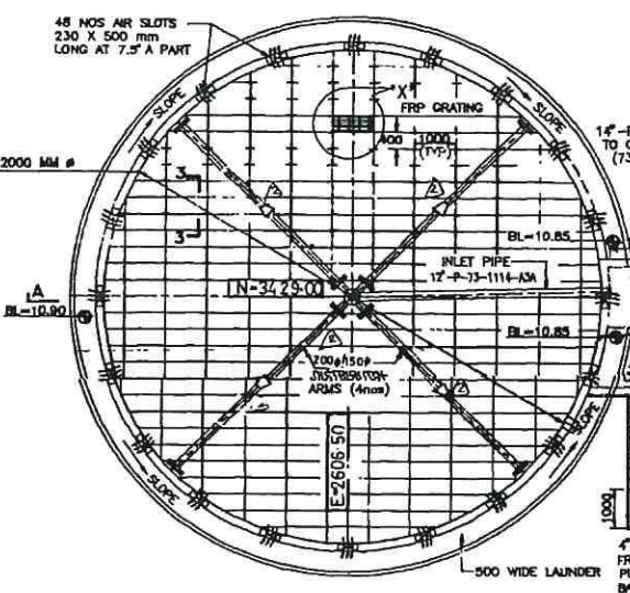
PLAN (SCALE 1:100)
