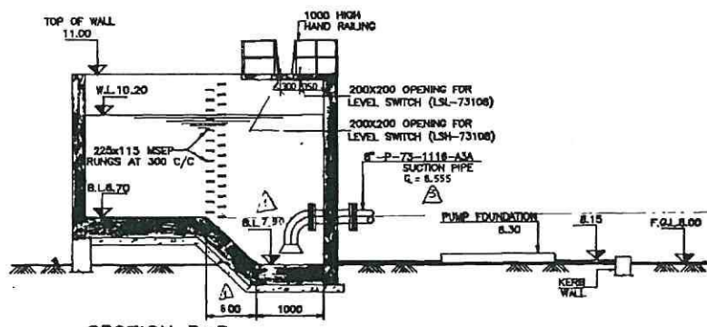
SECTION B-B (SCALE 1:50)
