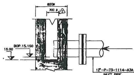
CENTRAL COLUMN DETAIL DETAIL-'Z' (SCALE 1:10)
