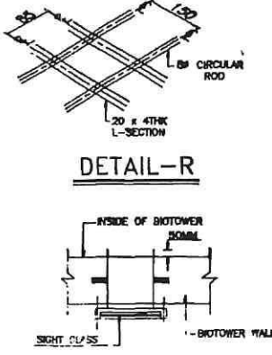
FIXING DETAILS OF SIGHT GLASS
