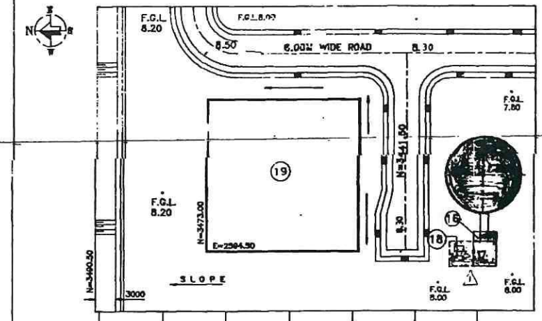
KEY PLAN (SCALE 1:100)
